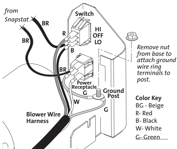
Figure 16. Wiring orientation.
