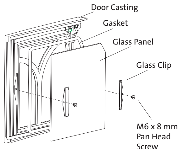
Figure 21b. Double Door Glass Assembly Parts.
