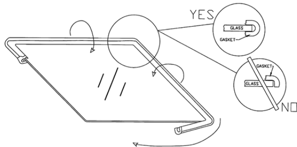
Figure 3 – Glass Gasketing
