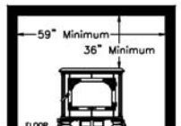
ALCOVE CLEARANCE TO COMBUSTIBLES
