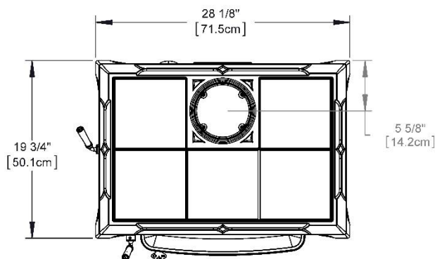
Figure 1 – Top View
