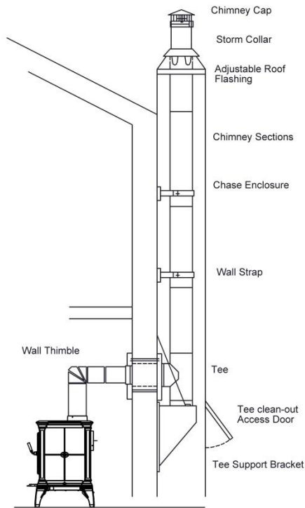
Chimney through outer wall with enclosed chase.
