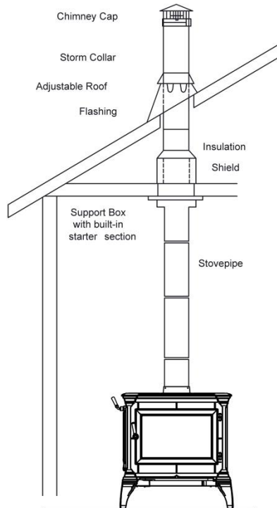
One story house installation with attic.
