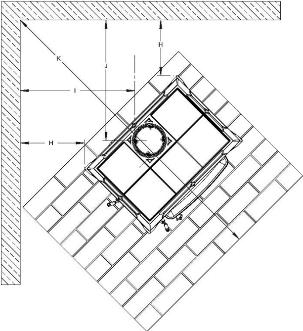
Figure 7 – Corner Clearances
