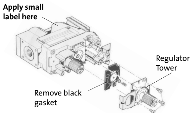
Figure 26. Regulator assembly.
