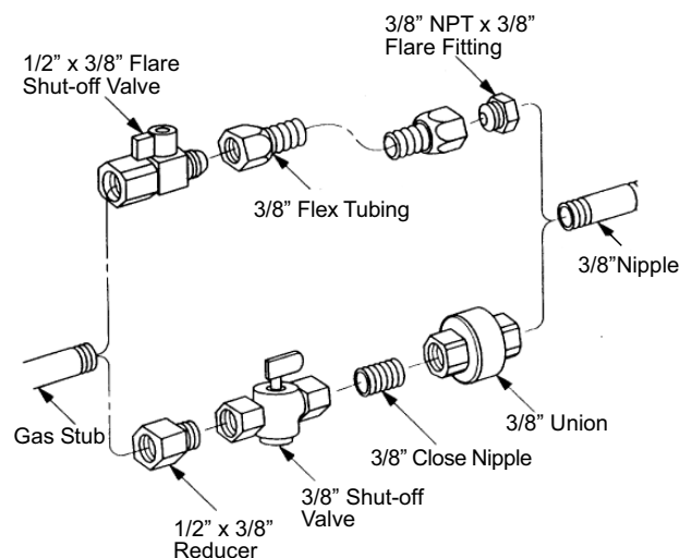
Figure 33. Supply valve connection fittings.
