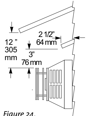
Figure 24. Termination Clearance to overhangs.
