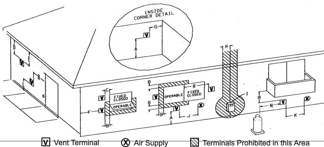
Figure 23. Vent Terminal Clearances, Canada and United States
