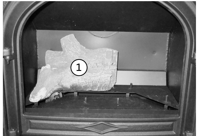
Figure 38. Engage the Left Logs with the two pins on the back shelf.
