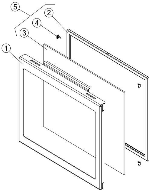
Figure 59. GF 200 DV IPI Glass Assembly
