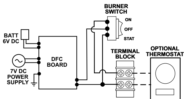
Figure 37. Accessory wiring diagram.
