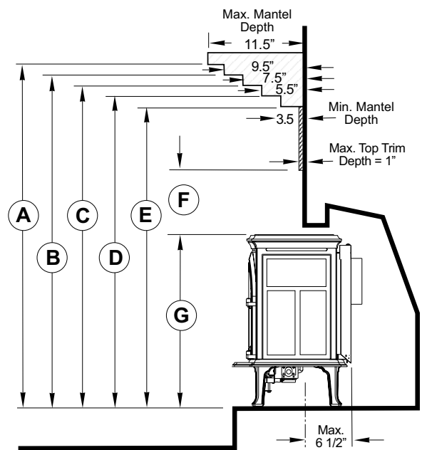
Figure 5. Mantel Clearances - stove flush with fireplace face. Add 2 1/4 inches to clearance if optional Long Leg Kit is used.
