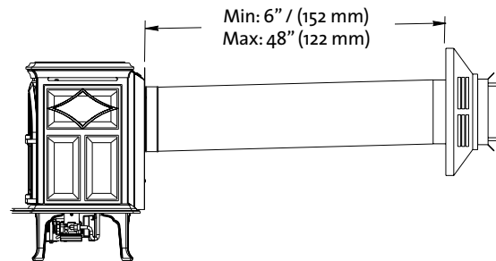
Figure 20. 5/8 Vent - Minimum / Maximum horizontal vent - no vertical run. 1/4 inch (6mm) rise per foot is required.
