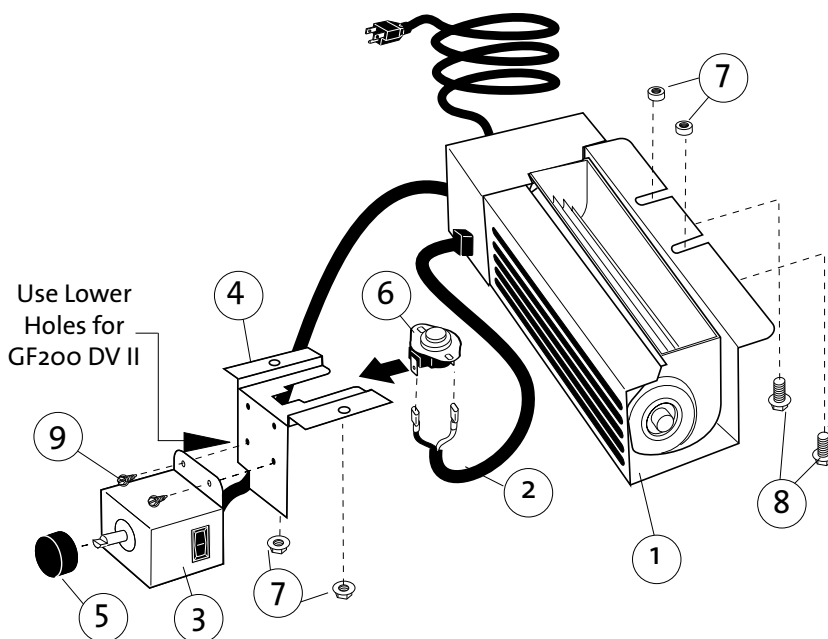
Figure 51. Blower Kit Components
