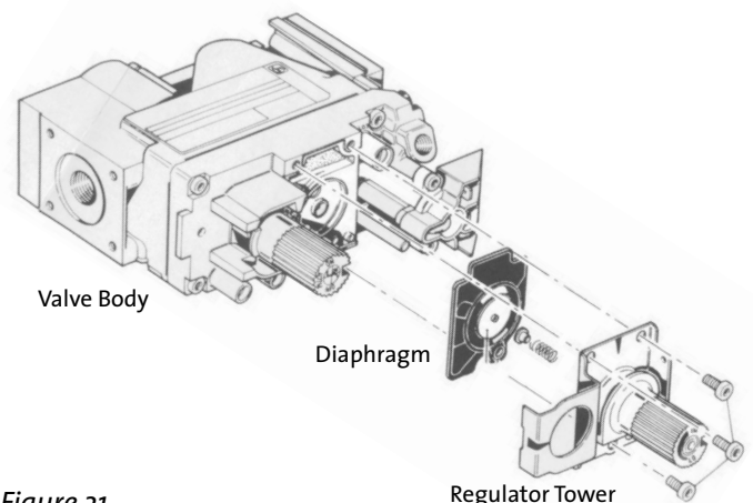
Figure 31. Regulator tower replacement.
