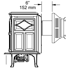
Figure 19. 4/6 Vent - Minimum / Maximum run for horizontal termination.
