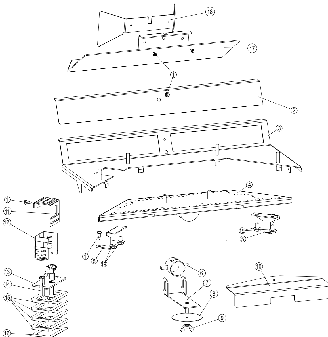
Figure 57. GF 200 DV IPI Pilot & Burner assembly and associated hardware.
