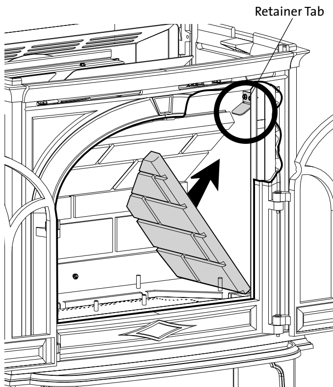
Figure 36. Install the Brick Panels.
