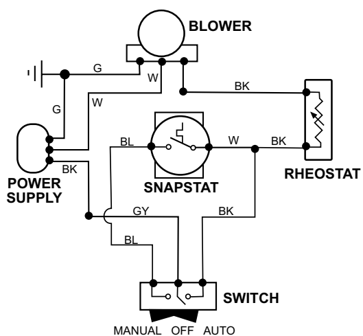
Figure 53. GF 200 DV IPI Blower Wiring Diagram.
