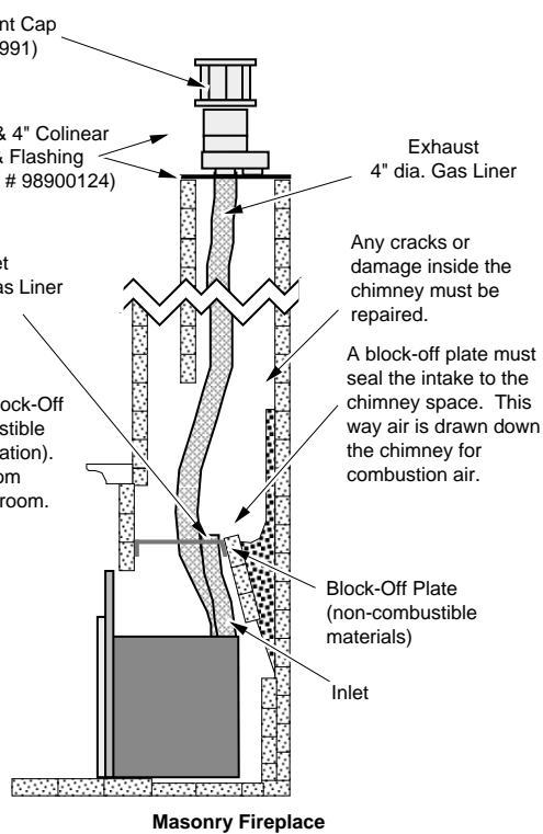
Masonry Fireplace
